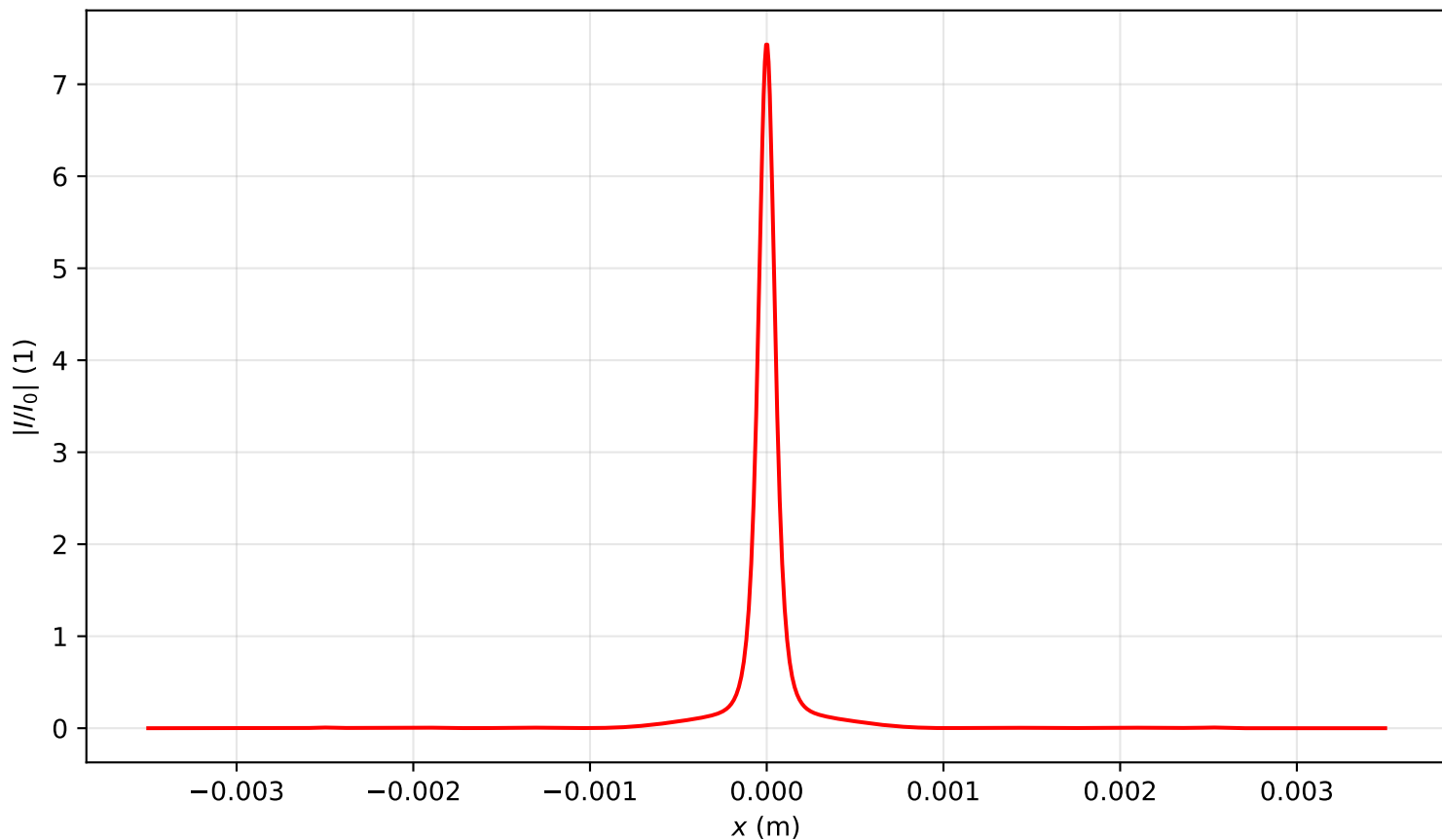
Intensity profile I(x, y = 0, z = 1.115)/I_0 , P_{in}=4.0P_{cr} , artificial time
